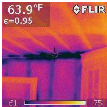
Dark spots are heat loss
