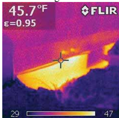
Heat loss around foundation
